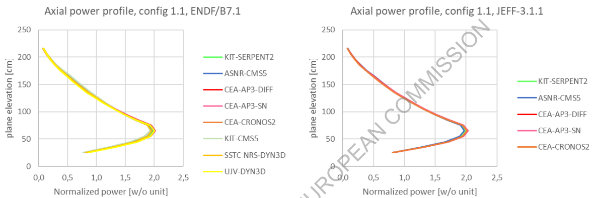
Figure 41. Power 1D axial profiles for config 1.1.
