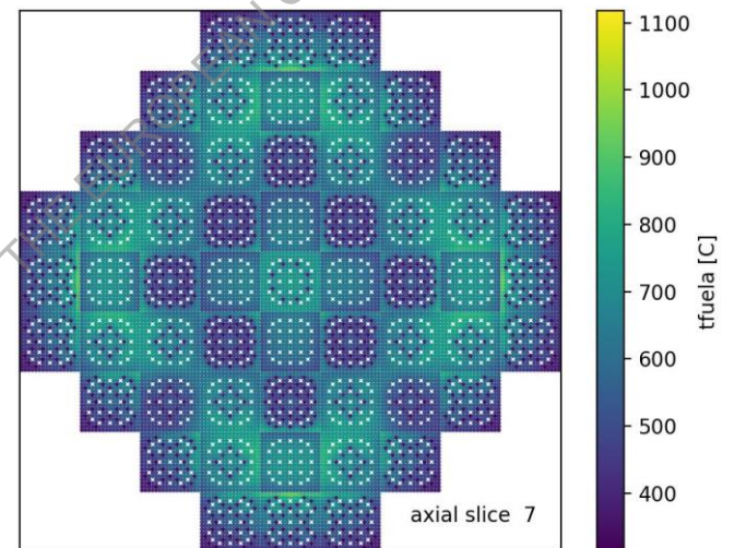
Figure 55. (Case 2.1, ENDF/B-VII.1) Serpent/SCF fuel temperature distribution in axial slice 7, corresponding to the peak-power region.
